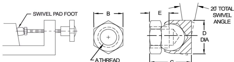
Steel Zinc Plated with Delrin® Pad
